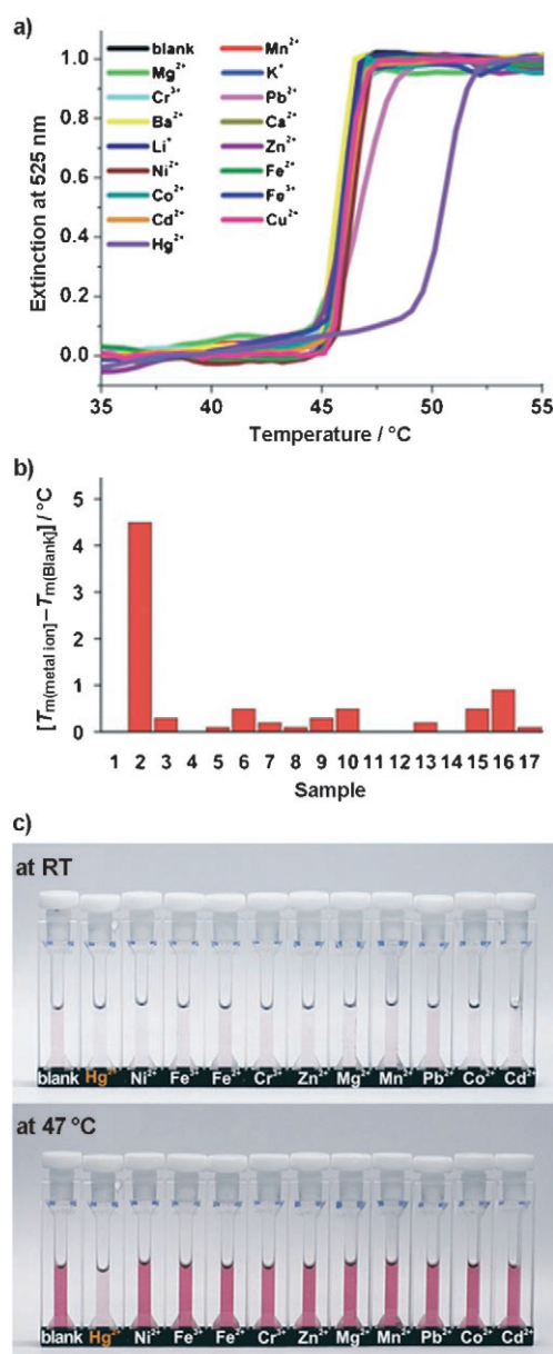
Figure 2. a) Normalized melting curves of the aggregates (probes A and B) in the presence of metal ions (each at 1 \mu\text{M} ). b) Graph showing the difference between the T_m of the aggregates of the blank and that of the aggregates with different metal ions: 1: blank; 2: \text{Hg}^{2+} ; 3: \text{Li}^+ ; 4: \text{Cd}^{2+} ; 5: \text{Ca}^{2+} ; 6: \text{Ba}^{2+} ; 7: \text{Mn}^{2+} ; 8: \text{Mg}^{2+} ; 9: \text{Zn}^{2+} ; 10: \text{Ni}^{2+} ; 11: \text{Fe}^{2+} ; 12: \text{Co}^{2+} ; 13: \text{Fe}^{3+} ; 14: \text{K}^+ ; 15: \text{Cr}^{3+} ; 16: \text{Pb}^{2+} ; 17: \text{Cu}^{2+} . c) Color change of the aggregates (probes A and B, each at 1.5 \mu\text{M} ) in the presence of various representative metal ions (each at 1 \mu\text{M} ) upon heating from room temperature (RT) to 47 ^\circ\text{C} . The colorimetric results for \text{Cu}^{2+} are not shown, as the data were taken after initial submission of the manuscript; see the Supporting Information.
